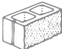
20.01 SF Full Block 400x200x200 108 per pallet
